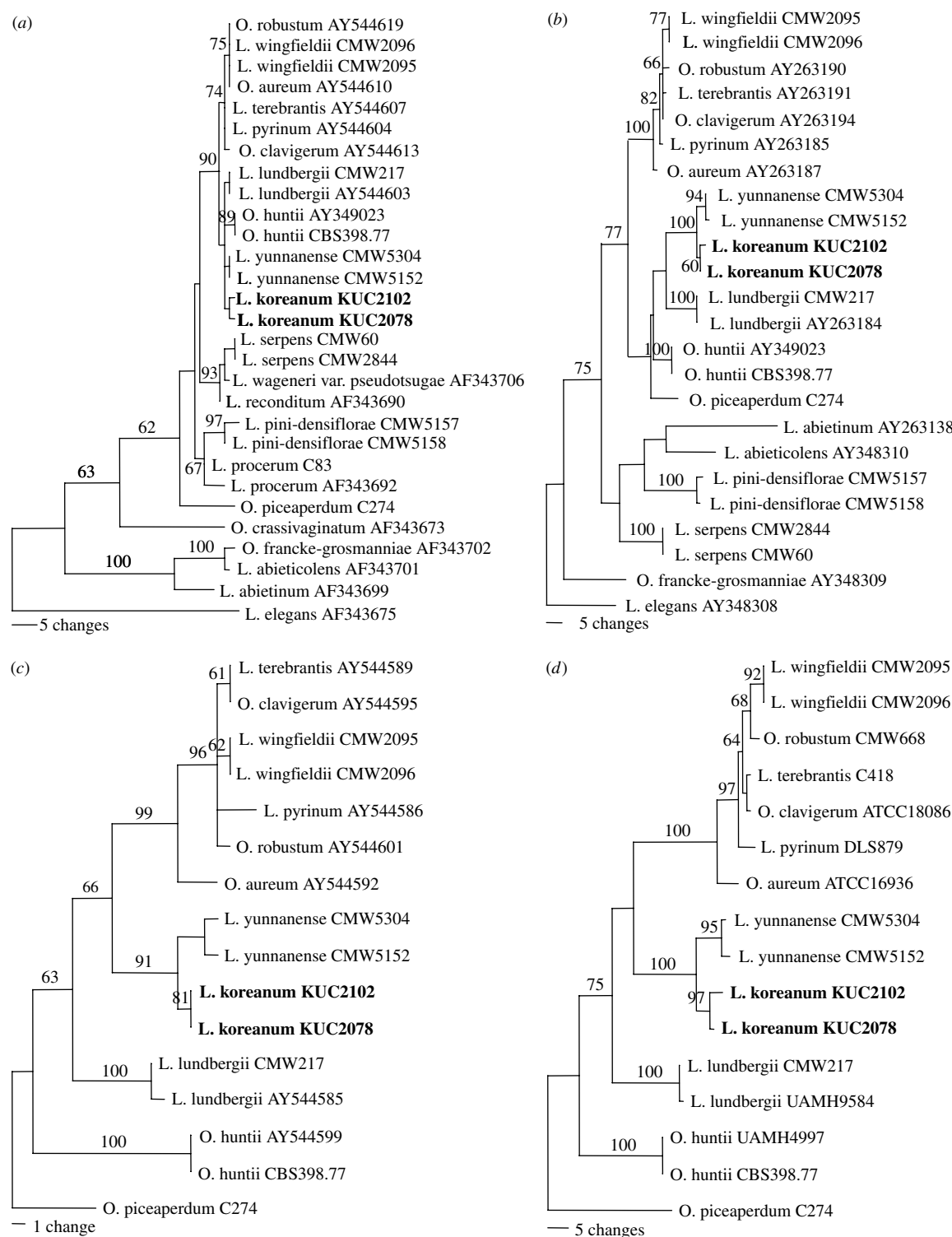
Fig. 7. Most parsimonious trees for each of the three nuclear gene datasets and the combined datasets: (a) rDNA, (b) \beta -tubulin, (c) actin, and (d) combined. Numbers above or below the branches are bootstrap values of MPT shown when greater than 60%.
